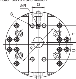
FA-610 單斜契式傳動 (配合伺服傳動) FA-812 WEDGE PLUNGER (Able to match servo transmission)
